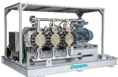
High-pressure Reciprocating Pump (Diaphragm)
