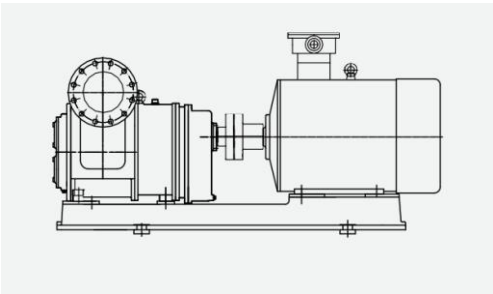
Concentric Installation Way of Integrated Gearbox
